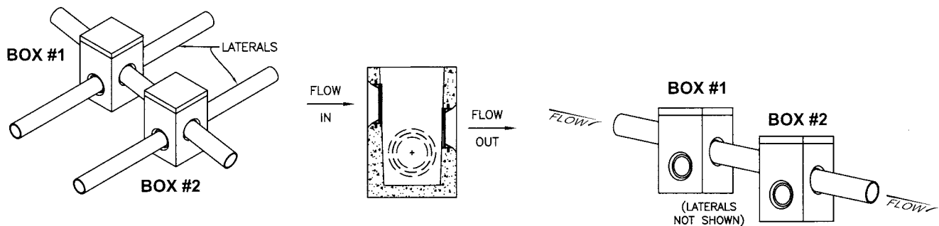
Step 2—Pumped System Installation
